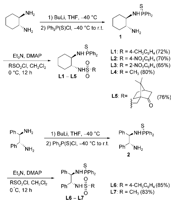
Scheme 1. Synthesis of sulfonamide-thiophosphoramidate ligands L1 – L7 .
